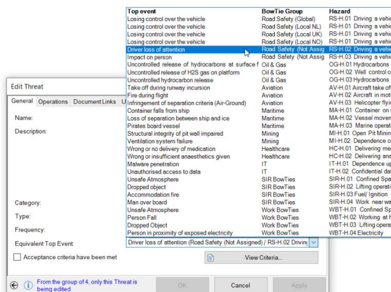
Figure 139 - Equivalent top event drop down
