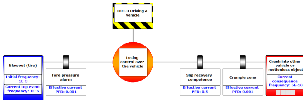
Figure 328 - Consequence frequency calculation via Classic LOPA: part 2
